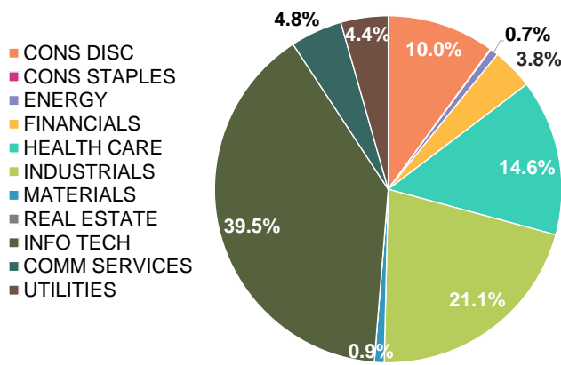
S&P Kensho New Economies Composite
