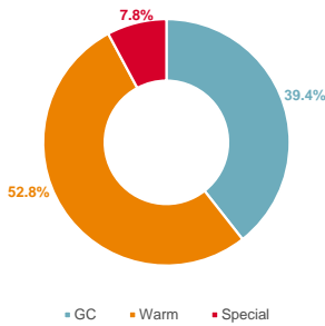
Annual Contribution by Fee Categories: Jun 24 to May 25
